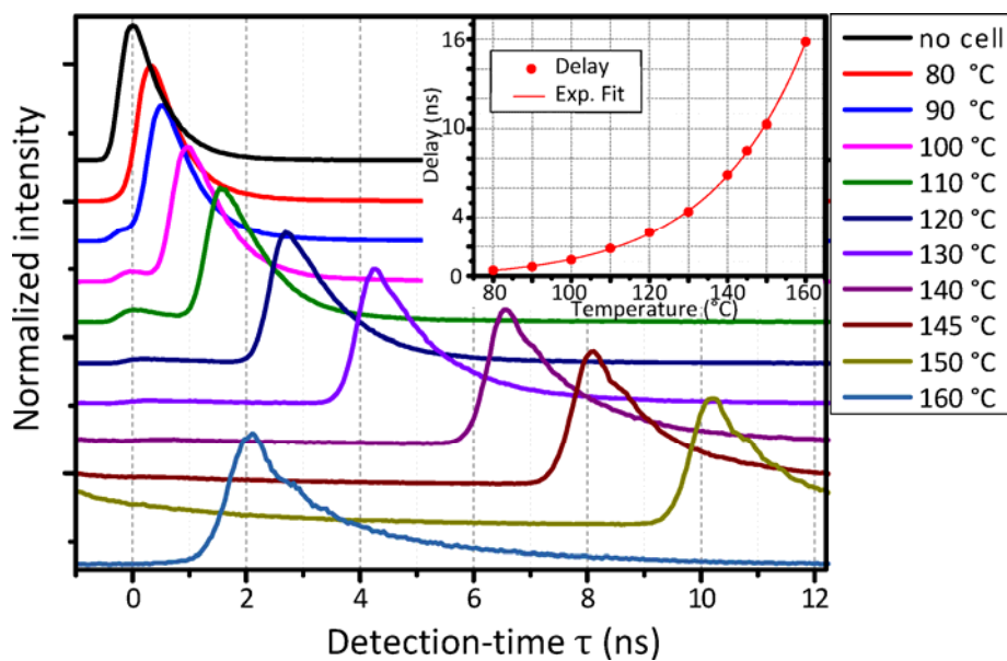
Fig.: Photon delay as a function of Cs-vapor temperature.
